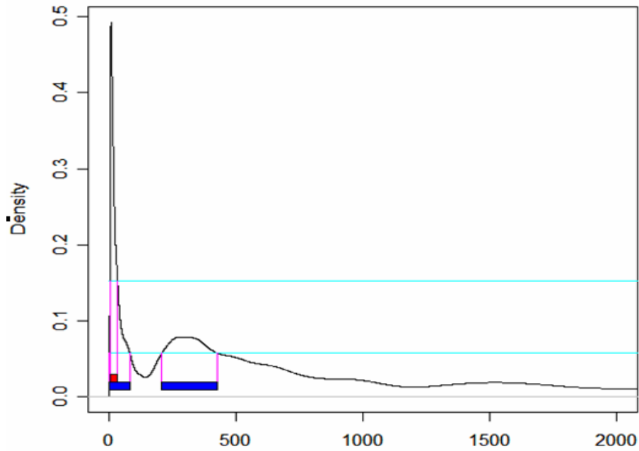
Figure 1. An example of density estimate of bootstrap distribution of half-life with 75% and 90% highest density regions.
