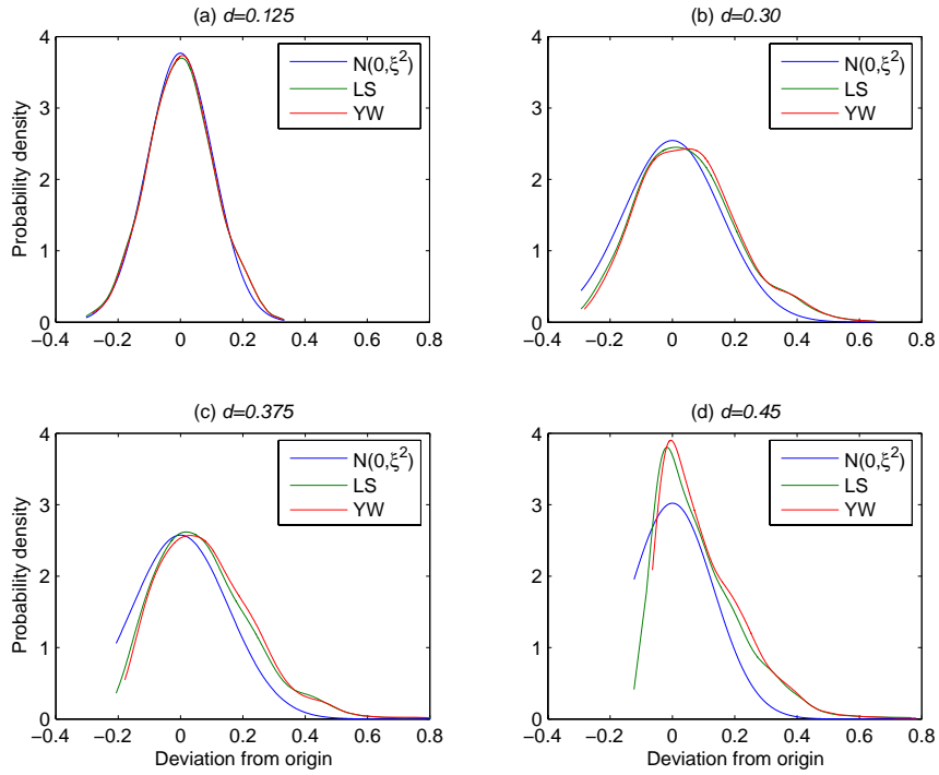
Figure 8: Empirical distribution of \sum_{j=1}^h (\hat{\phi}_h(j) - \phi(j)) for the fractional noise process y(t) = \varepsilon(t)/(1-z)^d with (a) d = 0.125 (b) d = 0.3 (c) d = 0.375 and (d) d = 0.45 , h = h_T^* = 1, 3, 4 and 5 respectively, and T = 100 .
