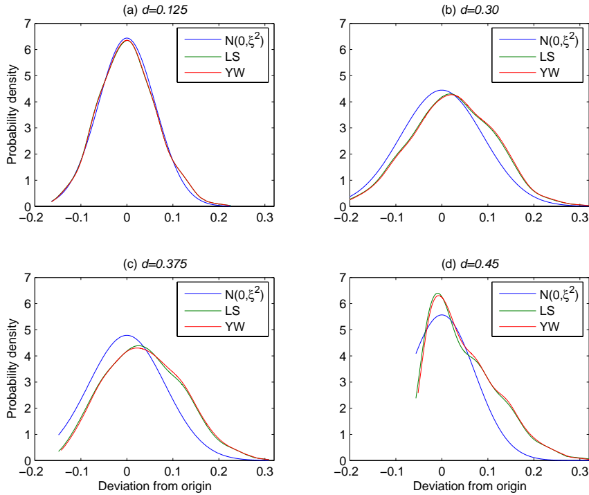
Figure 9: Empirical distribution of \sum_{j=1}^h (\hat{\phi}_h(j) - \phi_h(j)) for the fractional noise process y(t) = \varepsilon(t)/(1-z)^d with (a) d = 0.125 (b) d = 0.3 (c) d = 0.375 and (d) d = 0.45 , h = h_T^* = 2, 7, 8 and 10 respectively, and T = 500 .
