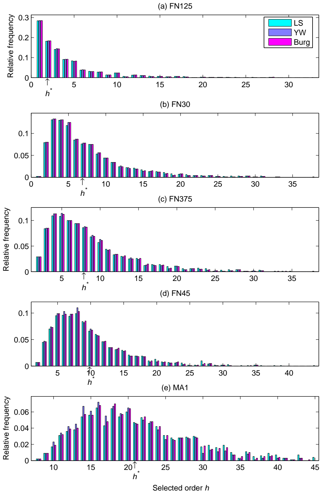
Figure 2: Relative frequency of occurrence of h_T^{AIC} , T = 500 , for the fractional noise process y(t) = \varepsilon(t)/(1 - z)^d with (a) d = 0.125 (b) d = 0.3 (c) d = 0.375 and (d) d = 0.45 and (e) the moving average process y(t) = \varepsilon(t) - \varepsilon(t - 1) .
