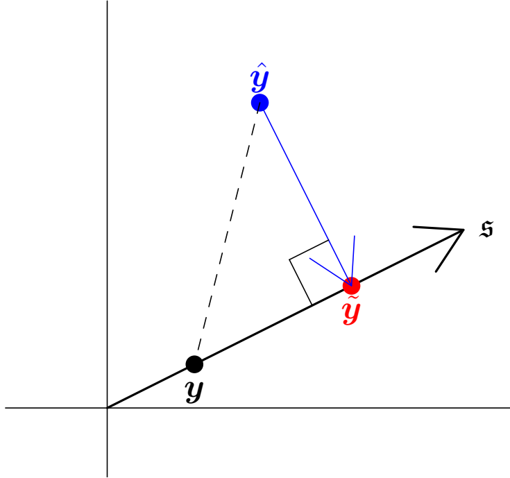
Figure 3: Orthogonal projection of \hat{y} onto \mathfrak{s} yielding the reconciled forecast \tilde{y} .
